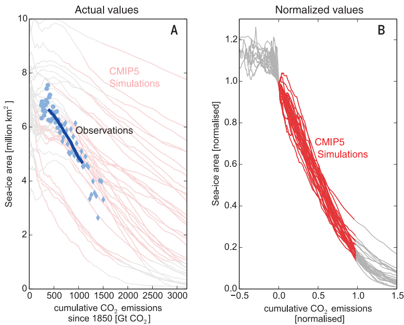
Fig. 1. Relationship between September Arctic sea-ice area and cumulative anthropogenic CO 2 emissions. (A) Actual values. The thick blue line shows the 30-year running mean of observed September sea-ice area, and the thinner red lines the 30-year running means from CMIP5 model simulations. For reference, we also show the annual values of observed September sea-ice area, based from 1953 to 1978 on HadISST (31) (circles) and from 1979 to 2015 on the NSIDC sea-ice index (32) (diamonds; see methods for details). (B) Normalized simulations. For this plot, the simulated CMIP5 sea-ice area is normalized by dividing by the simulated sea-ice area at the onset of the transition period as defined in the text. For each simulation, the cumulative emissions (33) are set to 0 at the onset of the transition period and then linearly scaled to reach 1 by the end of the transition period (compare table S1 for actual values). This linearization is only carried out to more explicitly visualize the linearity in the models. All analyses in the paper are based on the original data shown in (A).
