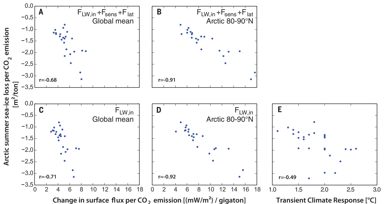
Fig. 3. Relationship between Arctic sea-ice loss and other metrics.
