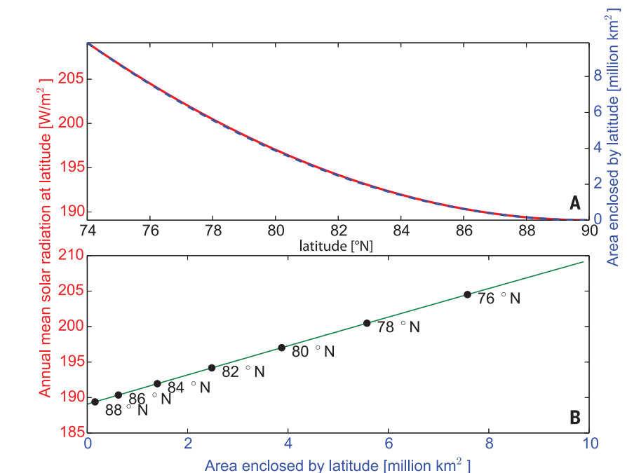
Fig. 2. Relationship between annual mean incoming shortwave radiation and sea-ice area. (A) Annual mean incoming top-of-the-atmosphere shortwave radiation at, and area within, a given latitude. The area within a given latitude band is calculated from simple spherical geometry. The latitudinal dependence of average daily incoming shortwave radiation at the top of the atmosphere is calculated from the very good approximation S(\varphi) = 1 - 0.482P_2(\sin(\varphi)) , where P_2 is the second Legendre polynomial (34). (B) As in (A), but with the x axis exchanged for clarity.
